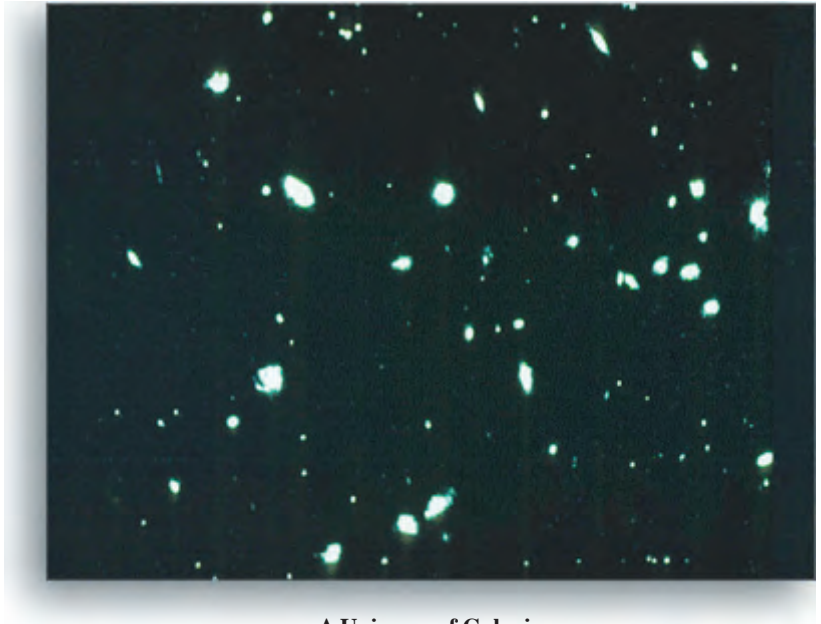
A Universe of Galaxies
