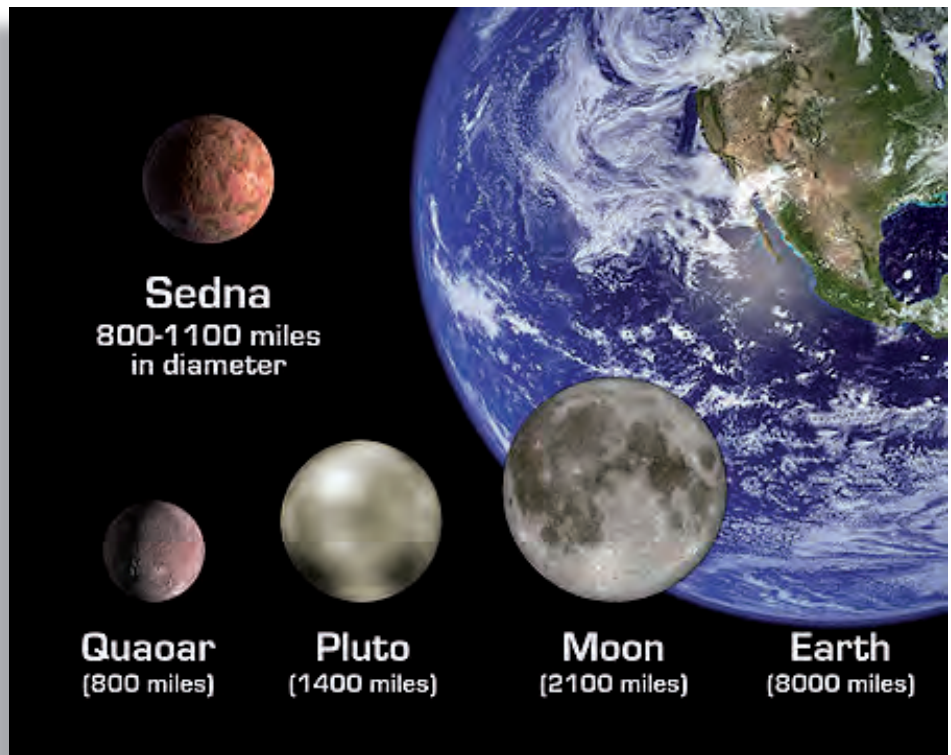
An artist's rendition comparing the size of the Earth, Moon, Pluto, Sedna and Quaoar. (Illustration Courtesy of NASA)
