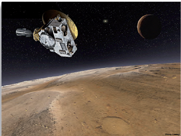
Artist's Illustration of New Horizons as it arrives at Pluto (Courtesy of NASA)
