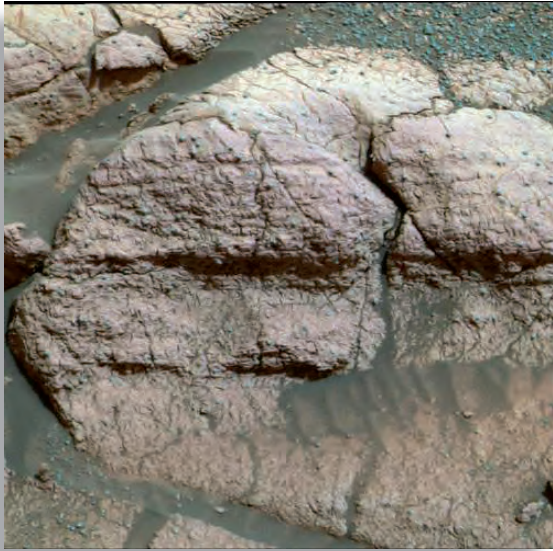
Photo confirmation of frozen liquid on Mars.
