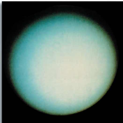
Color Image of Uranus Produced in 1986 (NASA)
