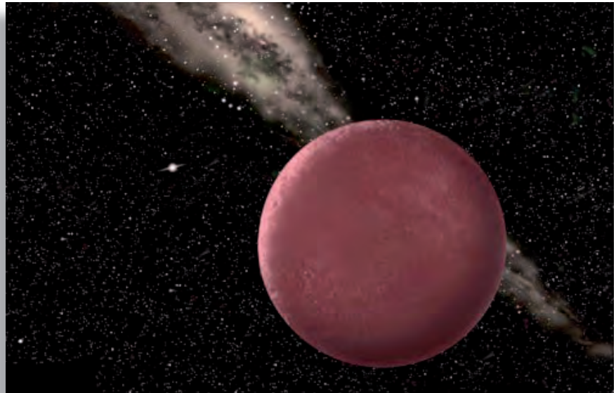
Bright red Sedna with the sun dimly seen in the distance. (Courtesy NASA)
