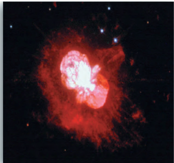
Supernova
