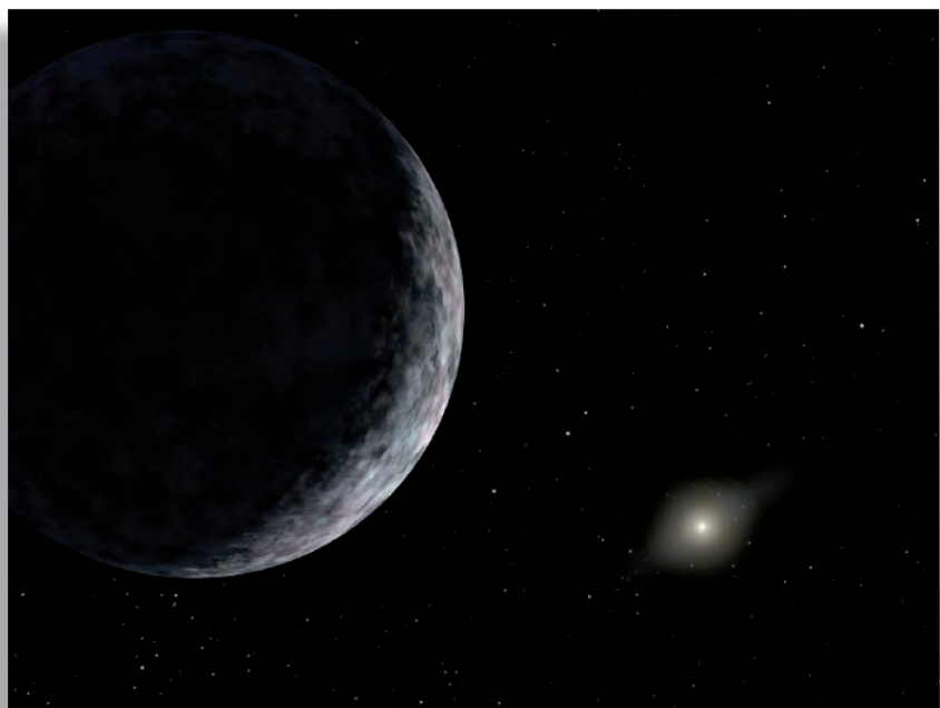
Artist’s concept of Eris with the Sun far away in the distance. (Courtesy NASA)
