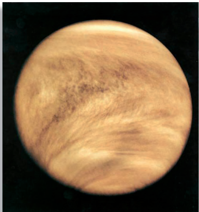
The Venus atmosphere as seen by ultraviolet imagery. (NASA Photo)
