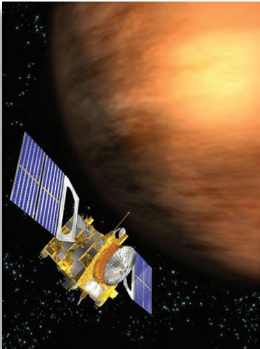
The probe Venus Express in orbit around the planet. (NASA Illustration)
