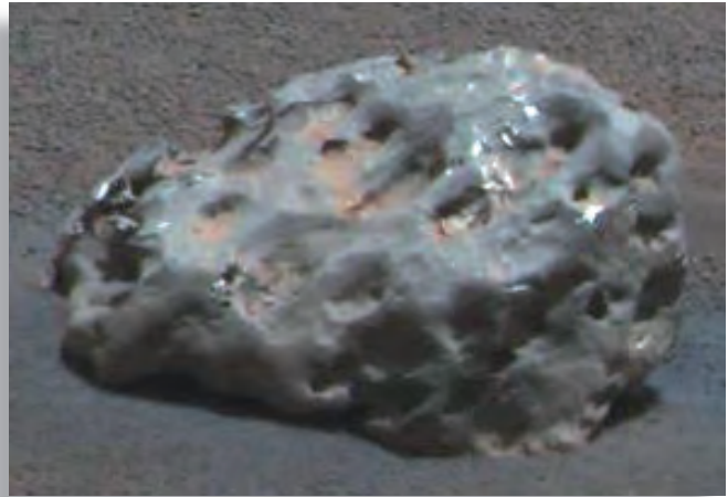
Opportunity discovered the first meteorite ever seen on Mars. (NASA)
