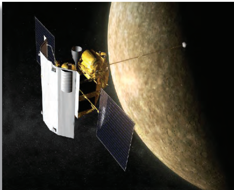
The Messenger satellite entering orbit around Mercury. (Illustration Courtesy of NASA)
