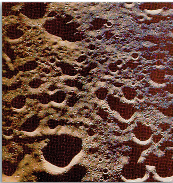
Moon Craters Taken by Apollo 8
