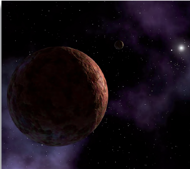
An Artist's Rendition Showing Sedna located in the Kuiper Belt. (Courtesy of NASA)
