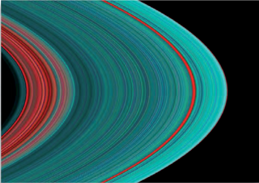
Icy Rings of Saturn (NASA)
