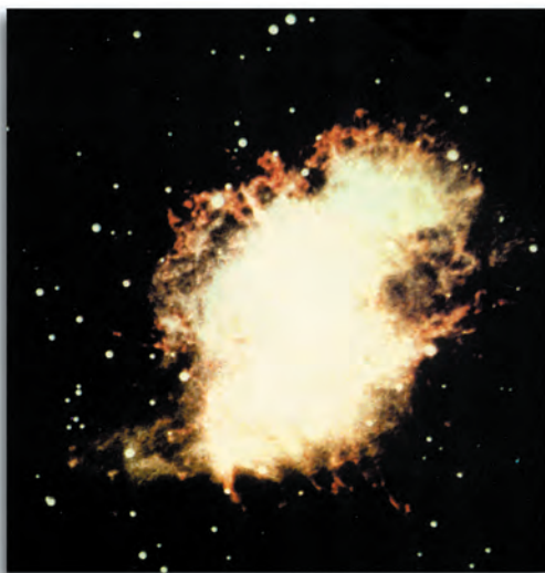
The Crab Nebula
