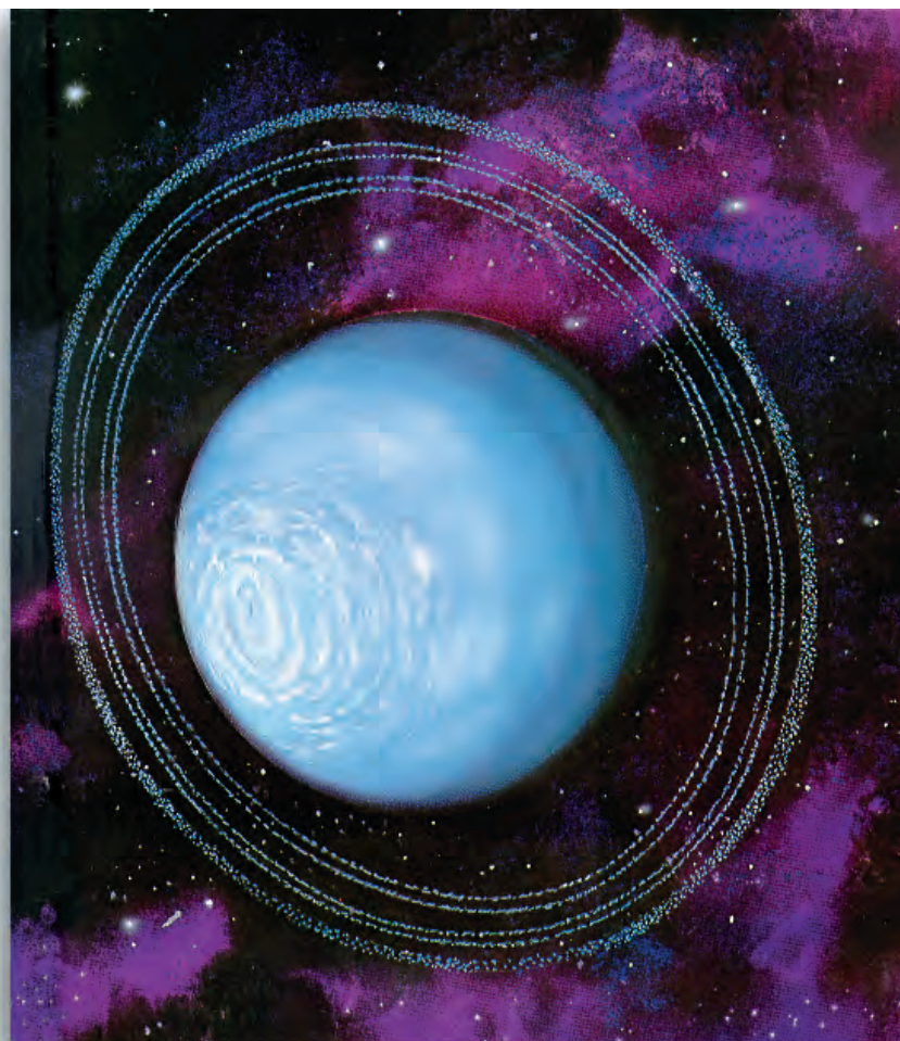
An Artist's Conception of the Rings of Uranus (NASA)
