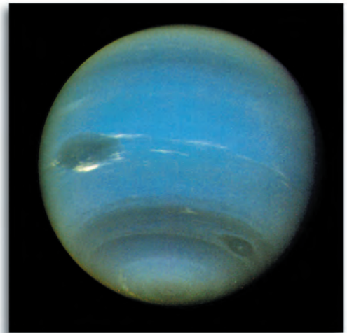
Neptune
