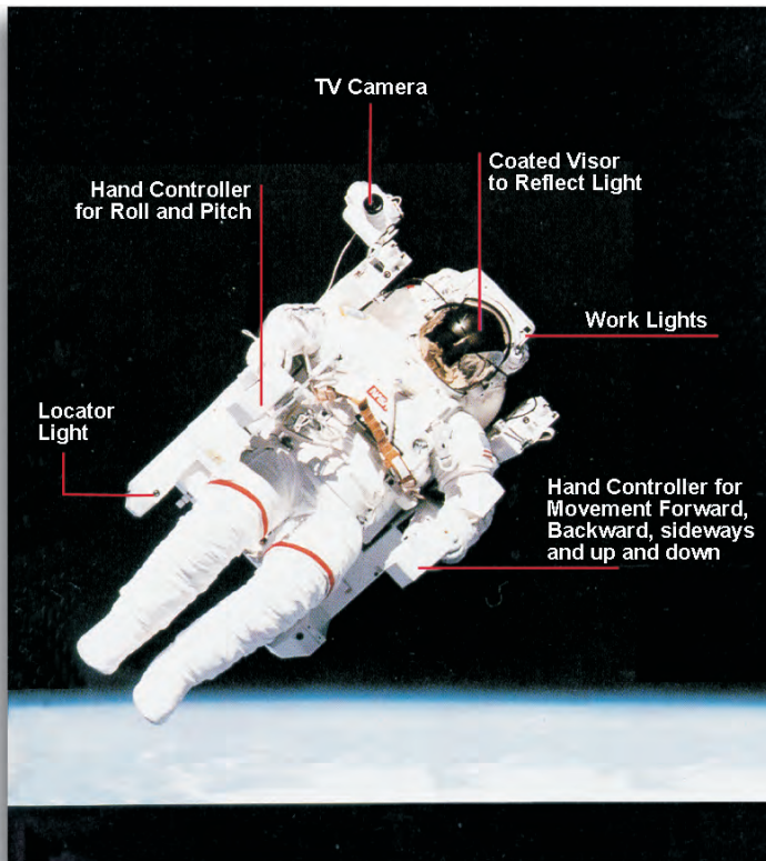
Manned Maneuvering Unit
