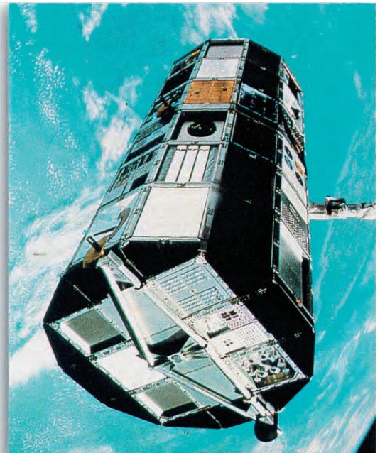
Long-Duration Exposure Facility (LDEF) during deployment from shuttle.
