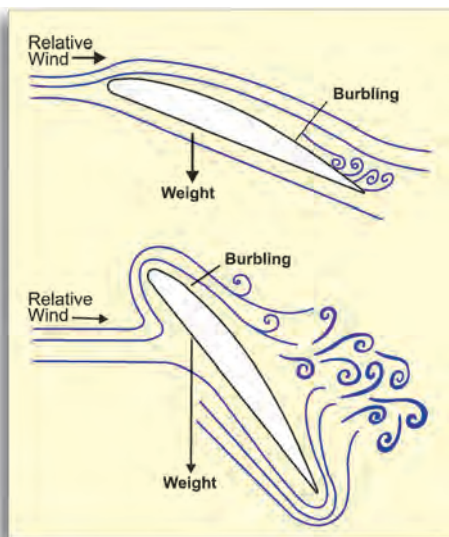
An airfoil approaching and entering a stall.
