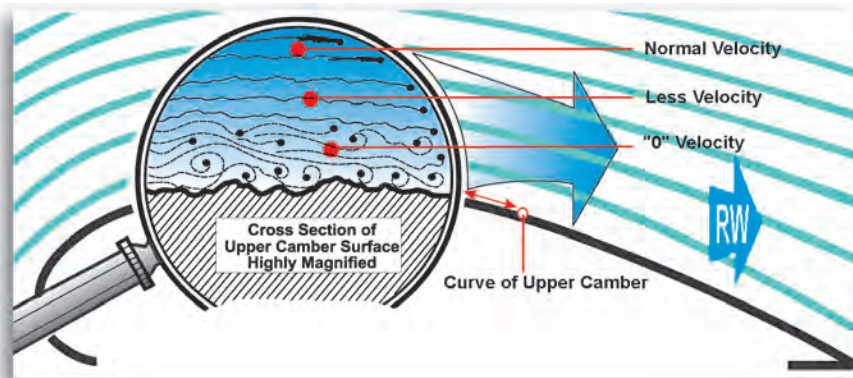
Friction Drag
